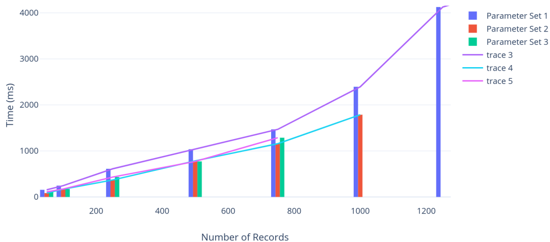
Figure 7.9: Graph : Number of records vs Delay time
